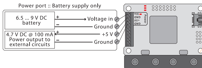
Figure 3 :: Battery power
