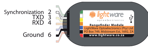
Figure 6 :: Serial interface connections
